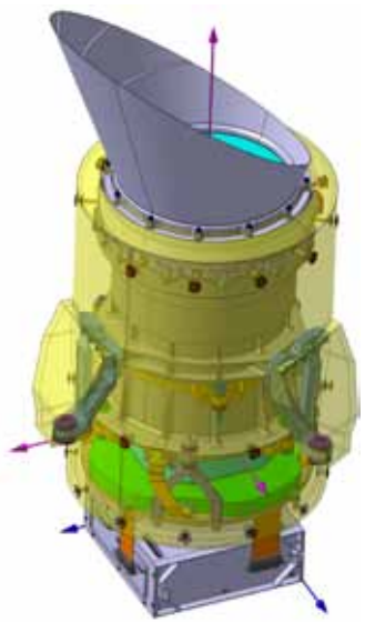
Schematic figure of one of the cameras of the PLATO spacecraft
